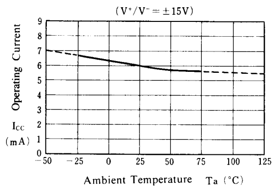
Operating Current vs. Temperature ( V^+/V^- = \pm 15V )
