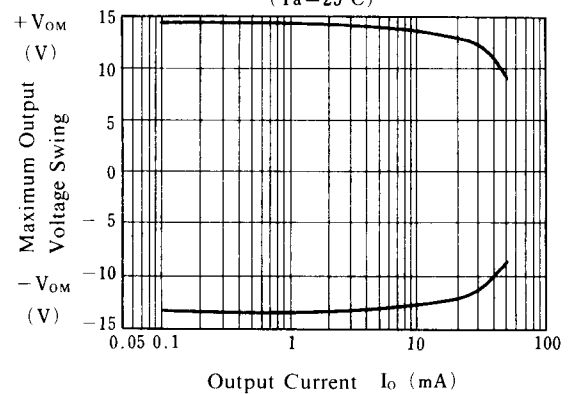
Maximum Output Voltage Swing vs. Output Current ( T_a = 25^\circ C )
